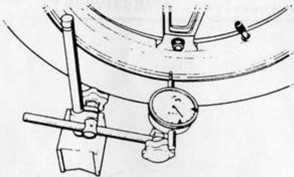
Radialt
